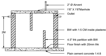
CROSS SECTION OF SEPTIC TANK
