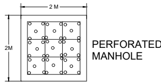
PLAN OF RAIN WATER RECHARGING PIT
