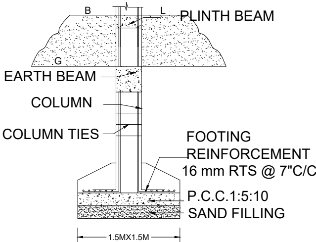
FOUNDATION DETAIL
