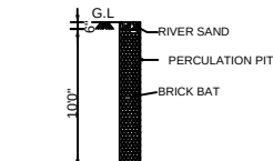
PERCOLATION PIT
