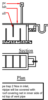
Tank With U Trap Not To Scale
