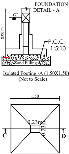
SECTION - 'CD'
