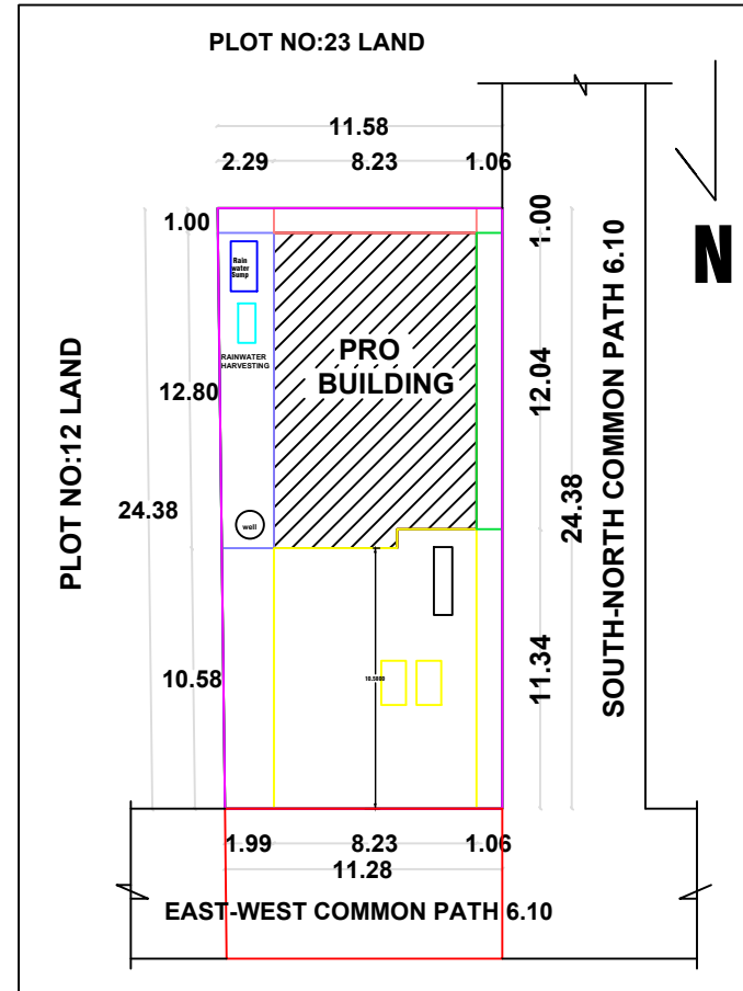
SITE PLAN & KEY PLAN (1:100)
