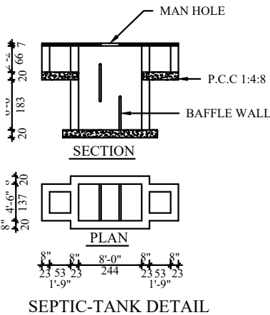
SEPTIC-TANK DETAIL
