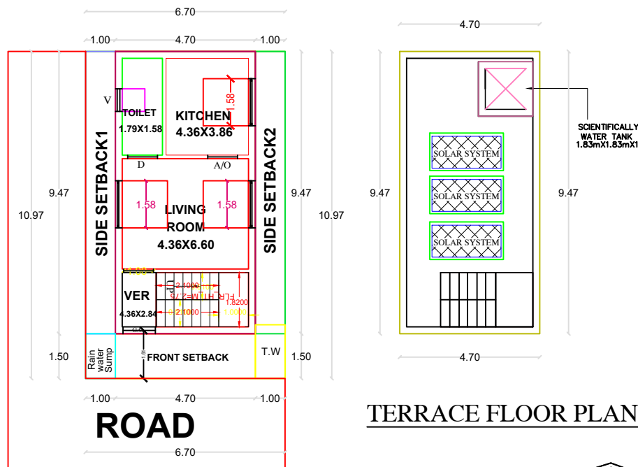
PLAN CUM GROUND FLOOR PLAN
