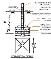
FOUNDATION DETAIL
