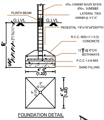
FOUNDATION DETAIL
