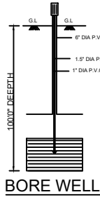
BORE WELL
