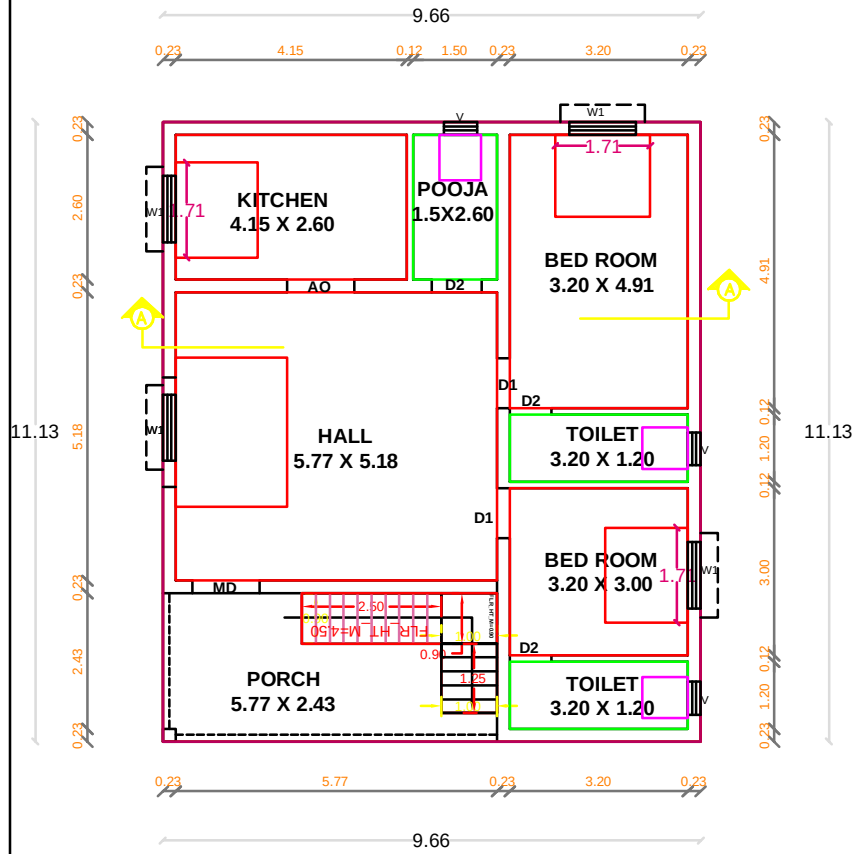
GROUND FLOOR PLAN PROPOSED
