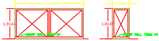
MAIN GATE ELEVATION WIKET GATE ELEVATION
