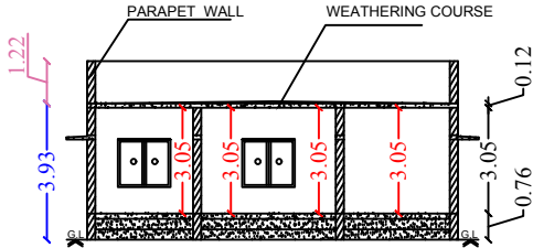
Section on-"AA"
