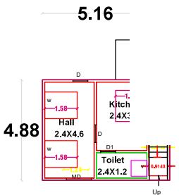
GROUND FLOOR PLAN TERRACE FLOOR PLAN
