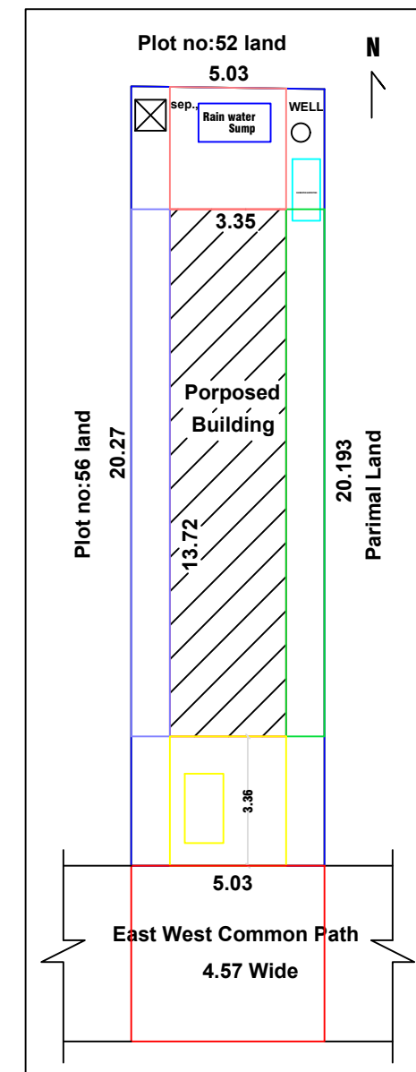
SITE PLAN CUM KEYPLAN
