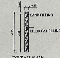
DETAILS OF PERCUSSION PIT
