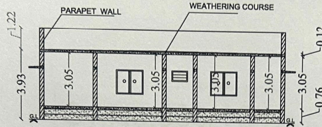
Section on-"AA"
