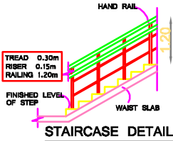
STAIRCASE DETAIL
