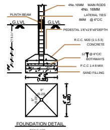
FOUNDATION DETAIL
