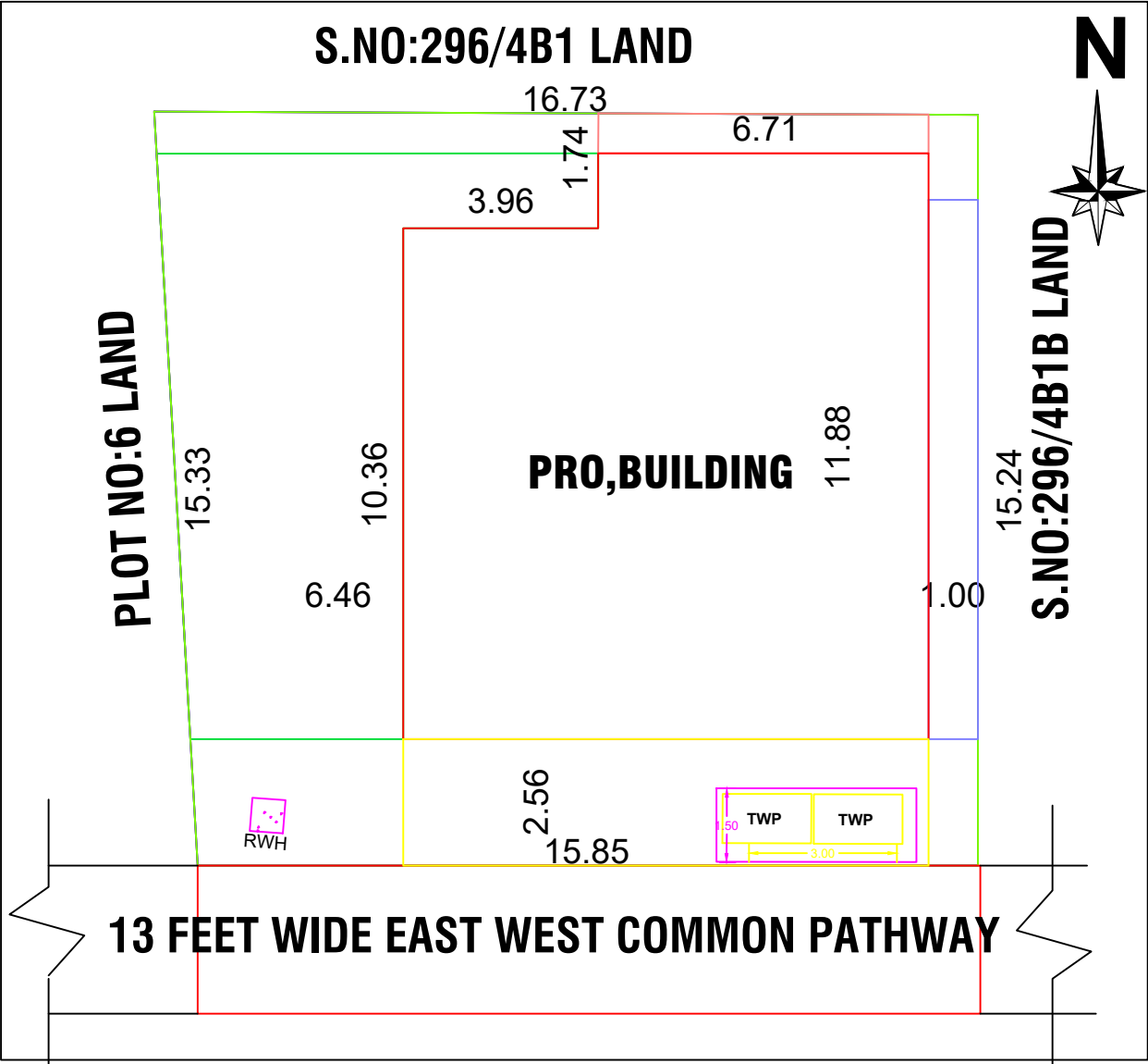
SITE PLAN
