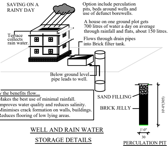
RWH_CAPACITY_L = 2000LTRS RAIN WATER COLLECTING TANK
