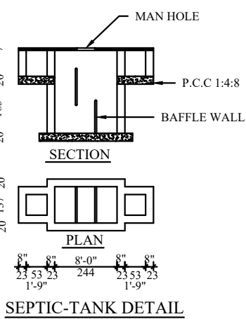
SEPTIC-TANK DETAIL
