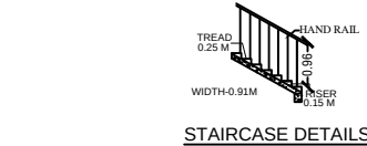
STAIRCASE DETAILS
