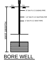
BORE WELL
