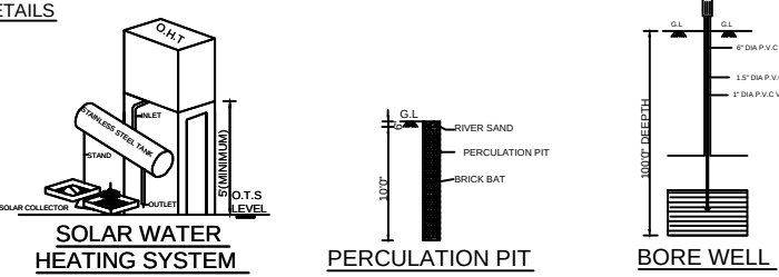
PERCOLATION PIT
