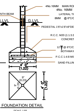
FOUNDATION DETAIL
