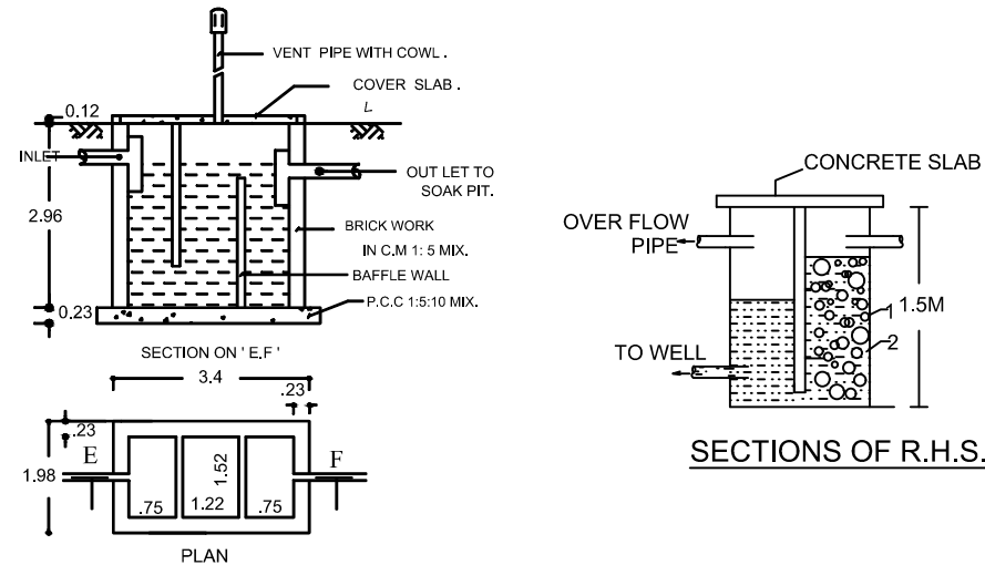
SEPTIC TANK DETAILS (NOT TO SCALE)
