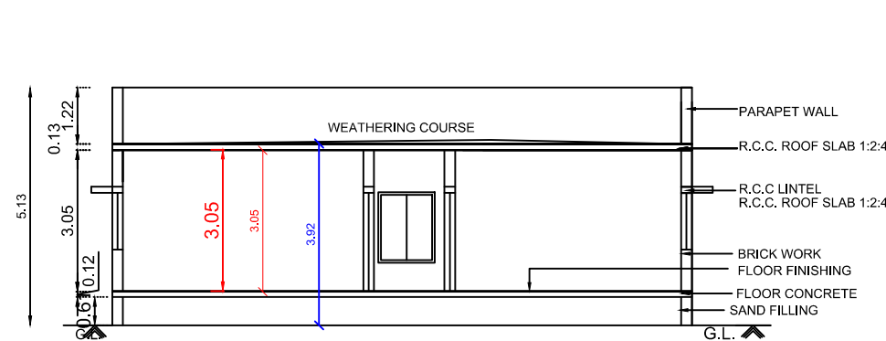
SECTION R-R
