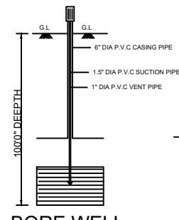
BORE WELL
