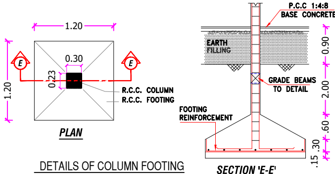
DETAILS OF COLUMN FOOTING
