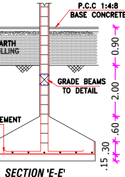
SECTION 'E-E'
