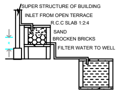
RAINWATER HARVESTING
