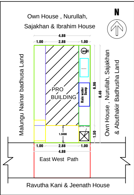
SITE PLAN & KEY PLAN
