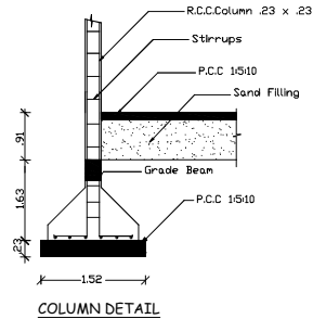
COLUMN DETAIL
