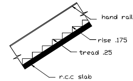
STAIR
