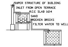
RAINWATER HARVESTING
