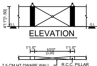
COMPOUND WALL PLAN
