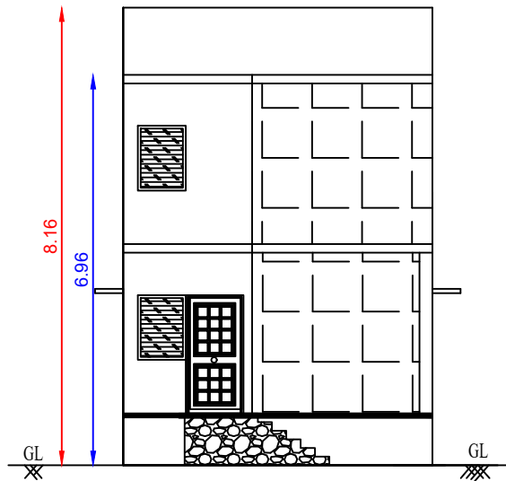
FRONT ELEVAION
