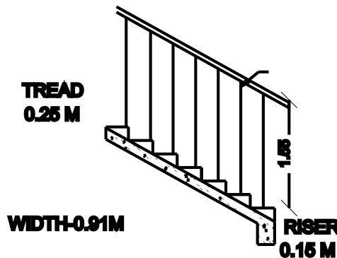
STAIRCASE DETAILS
