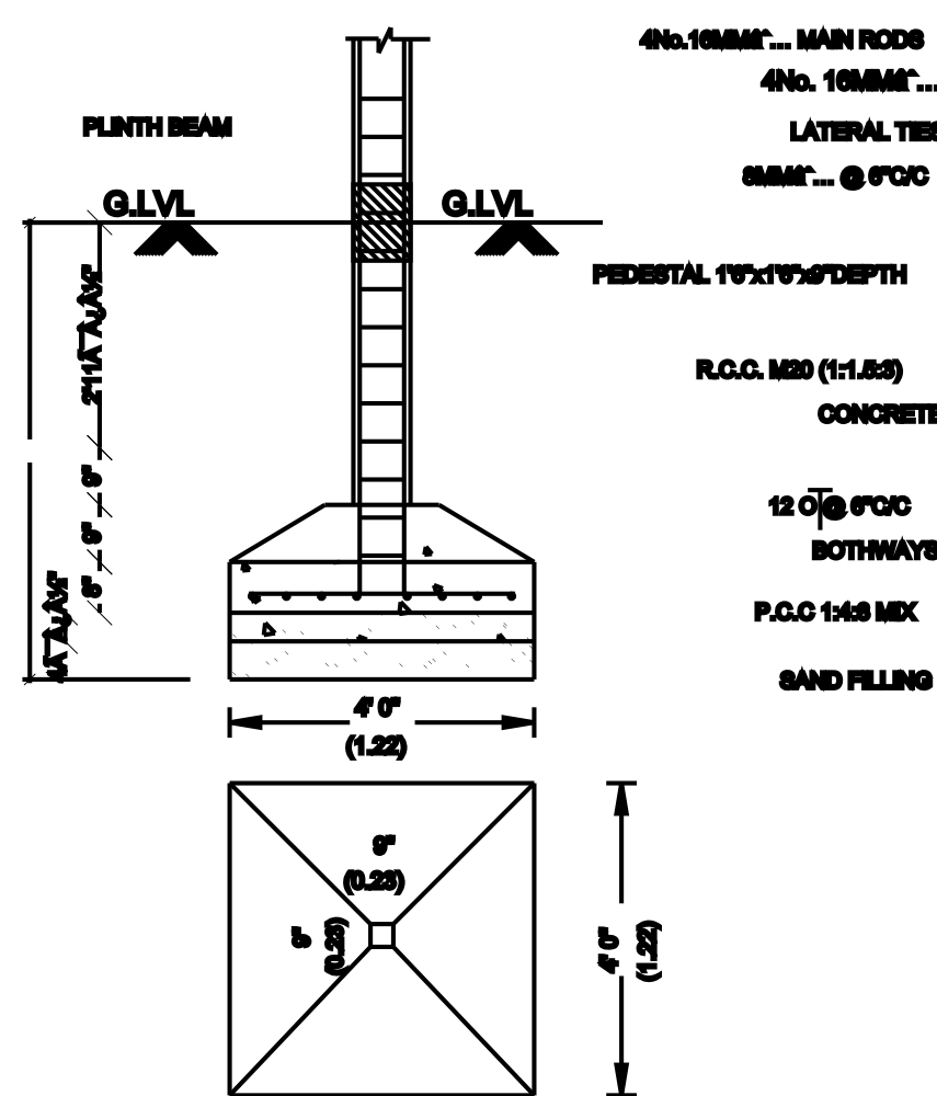
FOUNDATION DETAIL
