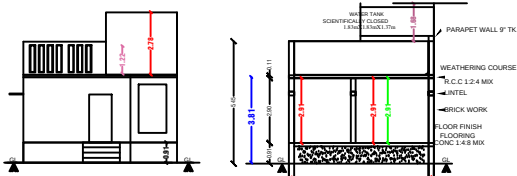
FRONT ELEVATION SECTION : "A-A"
