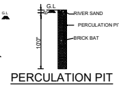
RAIN WATER HARVESTING SYSTEM
