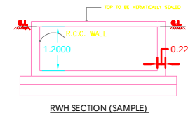
RWH CAPACITY L=2000LTRS
