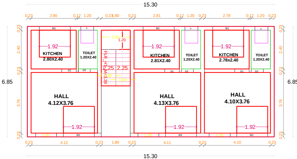
GROUND FLOOR PLAN PROPOSED
