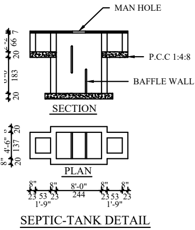
SEPTIC-TANK DETAIL
