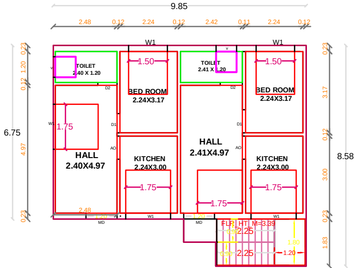
GROUND FLOOR PLAN PROPOSED
