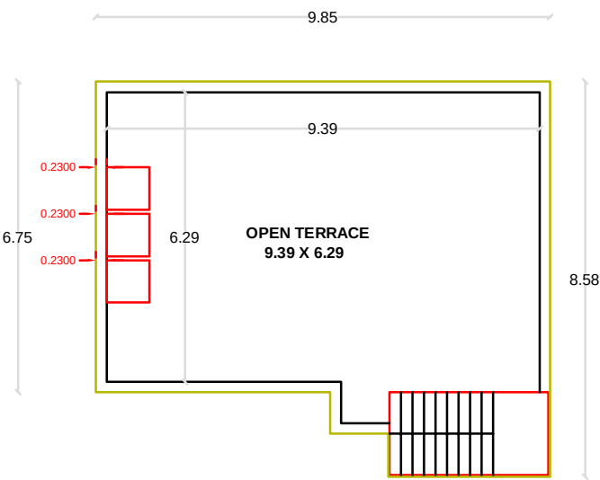
TERRACE FLOOR PLAN PROPOSED
