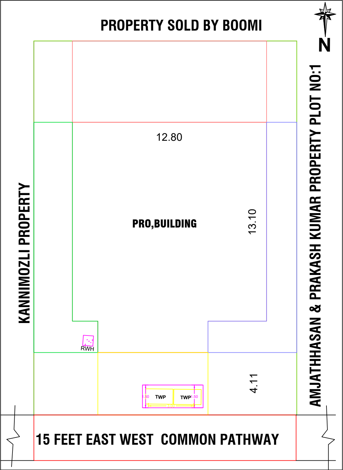
SITE PLAN
