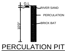
PERCOLATION PIT
