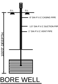
BORE WELL
