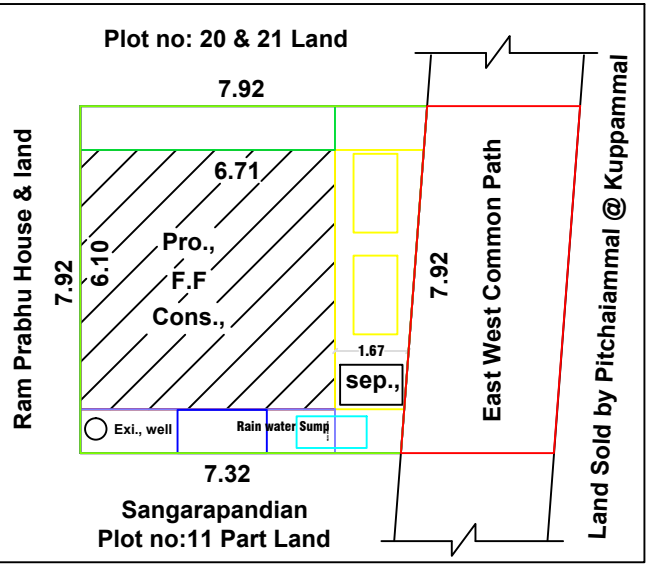
SITE PLAN & KEY PLAN (1:100)
