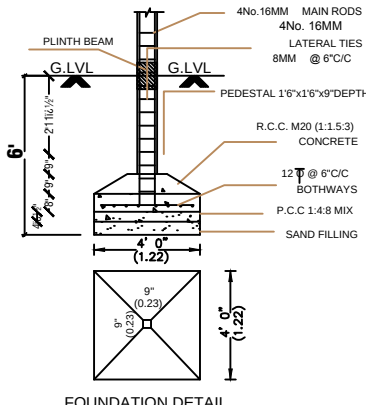
FOUNDATION DETAIL
