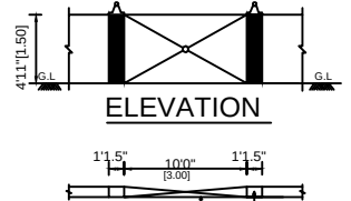
COMPOUND WALL PLAN
