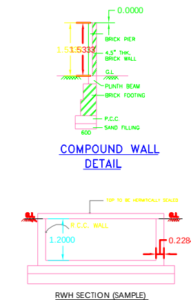
COMPOUND WALL DETAIL
