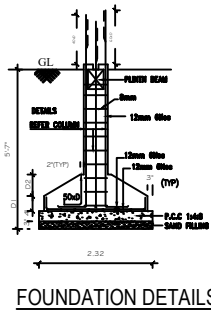
FOUNDATION DETAILS
