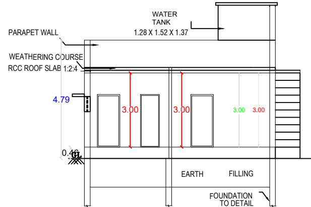
SECTION "A-B"
