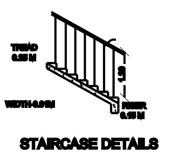
STAIRCASE DETAILS
