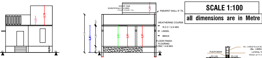
FRONT ELEVATION
