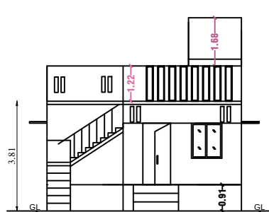
FRONT ELEVATION
