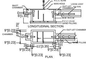
SEPTIC TANK:
