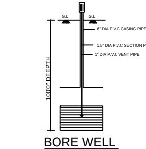
BORE WELL
