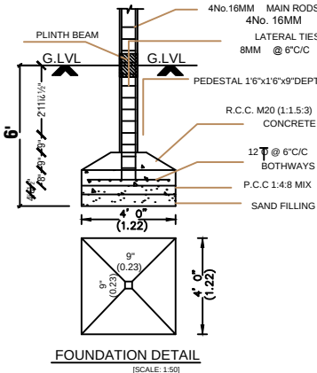
FOUNDATION DETAIL
