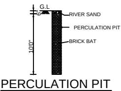
PERCOLATION PIT
