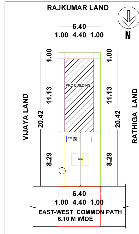
SITE PLAN & KEY PLAN
