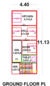
GROUND FLOOR PL
