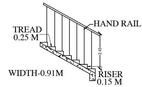
STAIRCASE DETAILS SECTION - CC
