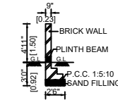
SECTION - CC
