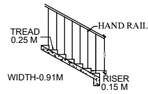
STAIRCASE DETAILS
