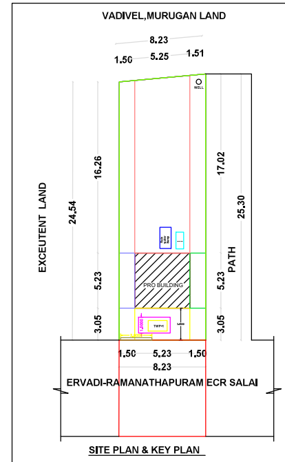
SITE PLAN & KEY PLAN
