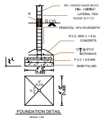
FOUNDATION DETAIL (SCALE 1:50)
