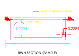
RWH_CAPACITY_L=2000LTRS
