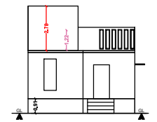
FRONT ELEVATION
