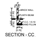
SECTION - CC
