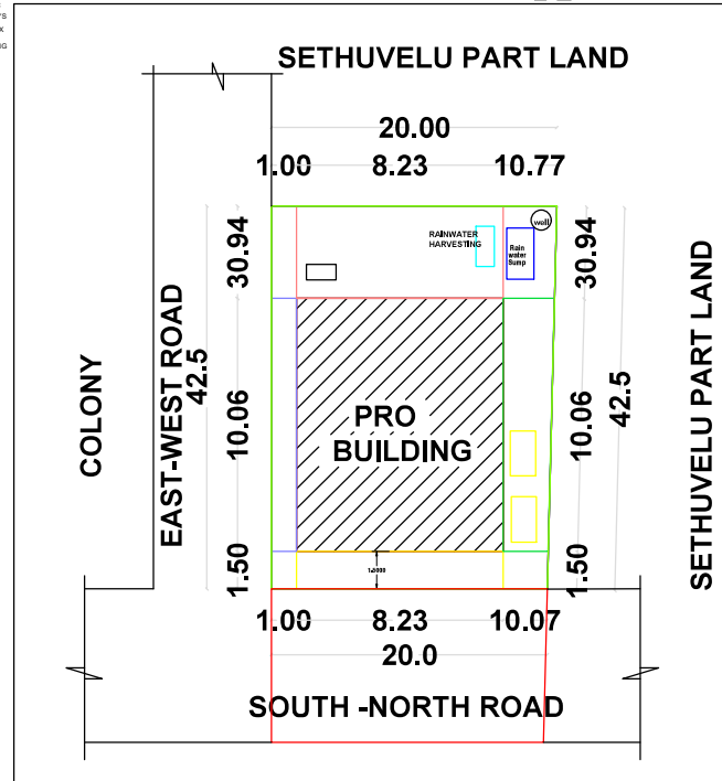
SITE PLAN & KEY PLAN (1:100)
