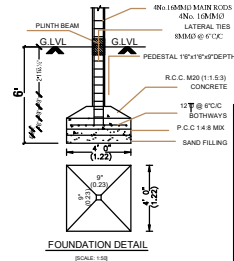
FOUNDATION DETAIL
