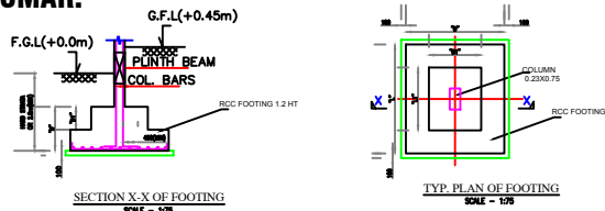
RCC COLUMN FOOTING DETAIL
