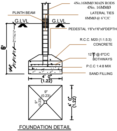
FOUNDATION DETAIL
