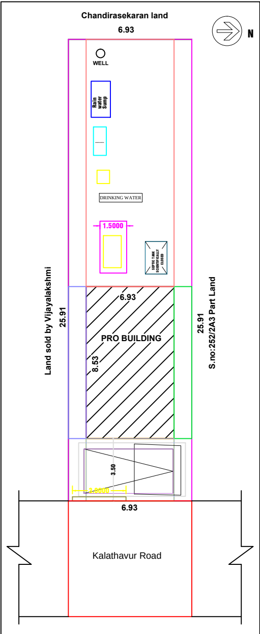
SITE PLAN & KEY PLAN
